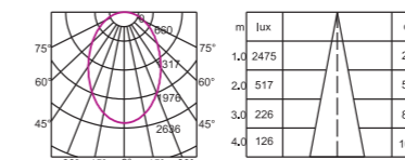
TL-MLL960 30W 4000K CRI>90 110°
