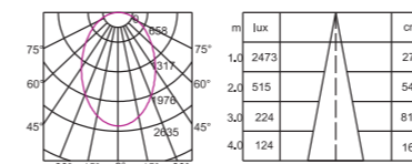
TL-MLL960 30W 3000K CRI>90 110°
