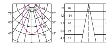
TL-SMGL3007 7W 4000K CRI>90 110°
